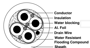
Cable Construction Relative Parts
