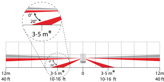
Figure 1: Range Adjustment
