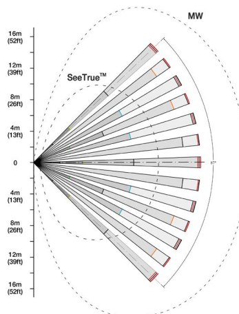
TOP VIEW (Forward Detector)
